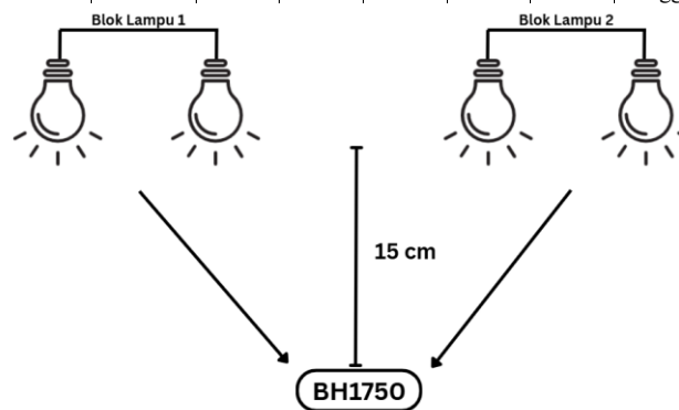
Fig. 3. Light Block Placement Scenario with BH1750 Sensor
